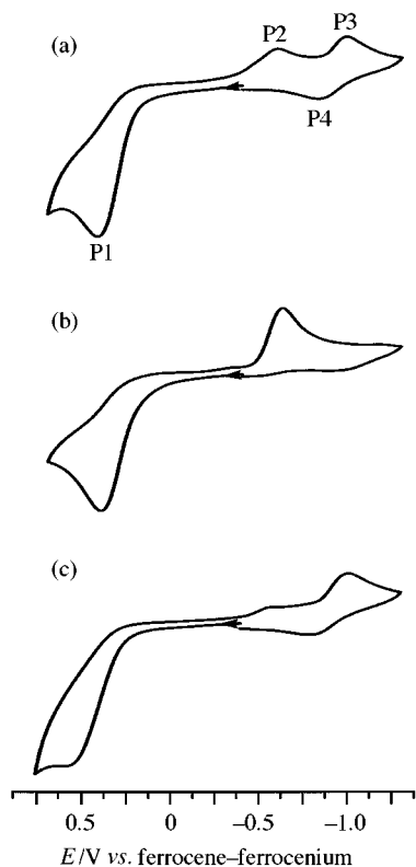
Fig. 6 Cyclic voltammograms (dmf–0.1 M \text{NBu}_4\text{NPF}_6 , 298 K, 100 \text{mV s}^{-1} ) of: (a) \text{H}_2\text{L}^3 \cdot \text{MeOH} ; (b) \text{H}_2\text{L}^3 \cdot \text{MeOH} + 3 mole equivalents of 2,6-dimethylpyridine; (c) \text{H}_2\text{L}^3 \cdot \text{MeOH} + 5 mole equivalents of water.
